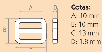
C10T Corredera de 10 mm
